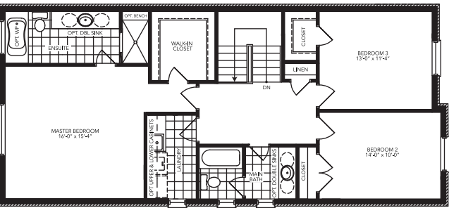
Second Floor Elevation A 3 Bedroom
