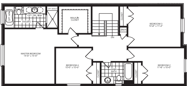
Second Floor Elevation A 4 Bedroom
